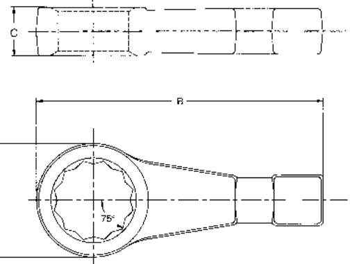
Roughneck "Hammer Wrench" Straight Pattern — 12 Point Alloy Steel — Drop Forged
