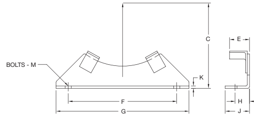
Saddle
