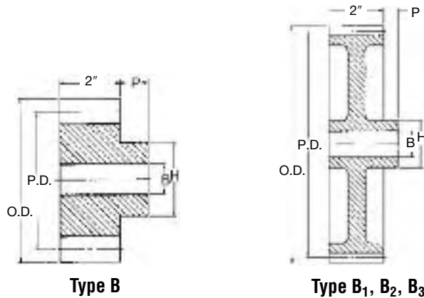
Type B 2 Web With Lighten Holes
