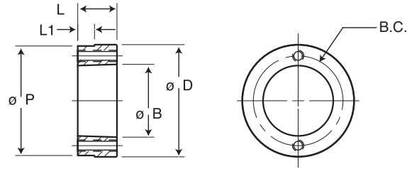
ALL TAPERS 3/4" PER FT. ON DIAMETER
